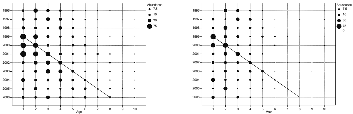
Figure 3. Age composition of ITQ survey indices by area (Scotian Shelf on left, Bay of Fundy on right) for 4X/5Y haddock. Solid line tracks 1998 yearclass.
