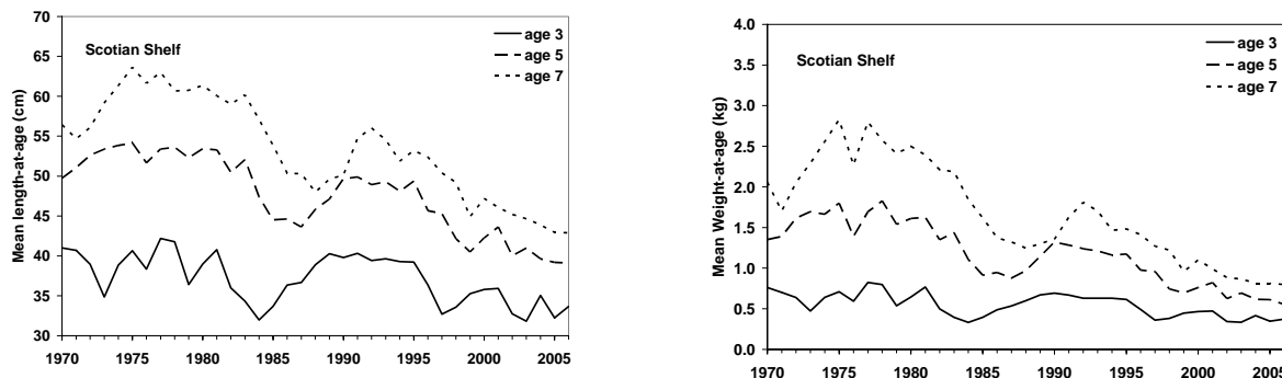
Figure 7. RV survey mean length-at-age (cm) (left) and mean weight-at-age (kg) (right) for 4X/5Y haddock.
