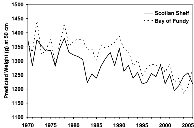
Figure 8. RV survey fish condition indices (predicted weight (g) at 50cm) by area for 4X/5Y haddock.
