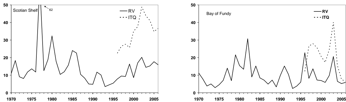
Figure 4. RV and ITQ survey 4+ biomass indices by area (Scotian Shelf on left, Bay of Fundy on right) for 4X/5Y haddock.
