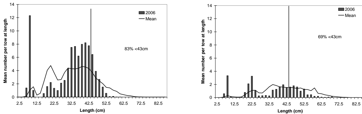
Figure 6. Length composition of 2006 RV survey catch (mean number per tow) compared to the long term mean (1970-2005). Vertical line indicates 43cm.
