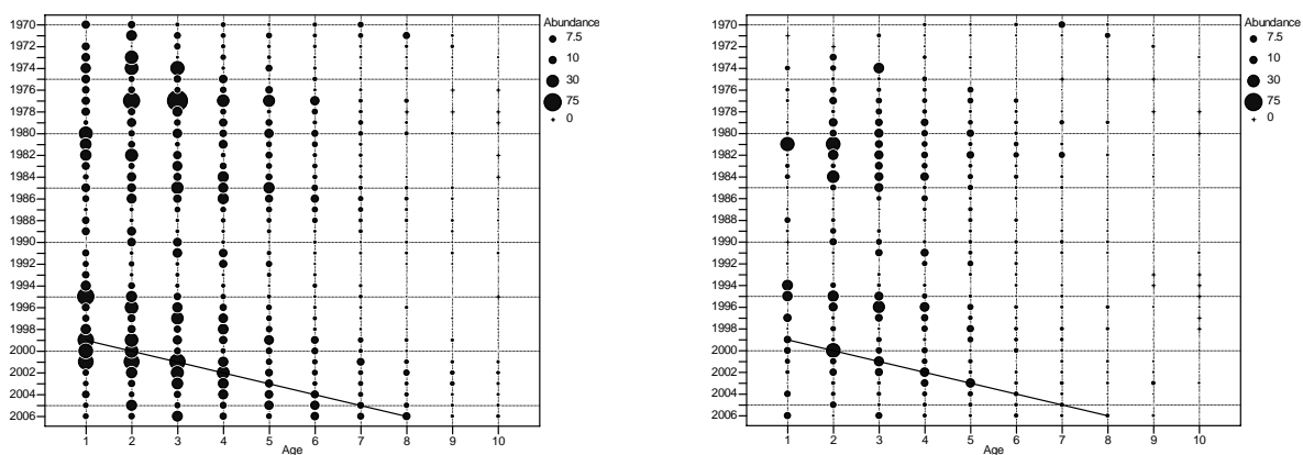
Figure 2. Age composition of RV survey indices by area (Scotian Shelf on left, Bay of Fundy on right) for 4X/5Y haddock. Solid line tracks 1998 yearclass.
