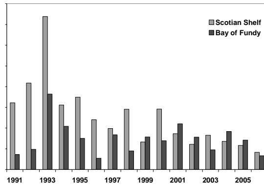
Figure 5. Relative fishing mortality by area in recent years for 4X/5Y haddock.
