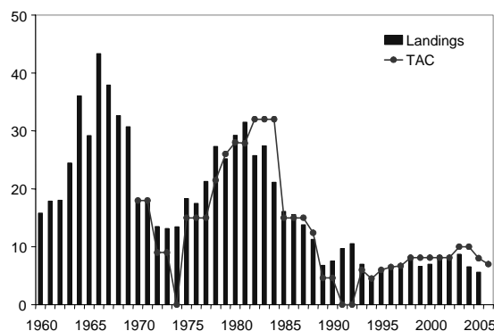
Figure 1. Landings* and TACs ('000t) for 4X/5Y haddock.
